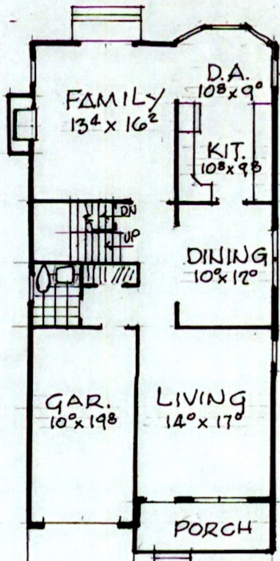
FIRST FLOOR
